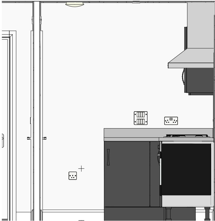
2 Kitchen - View B 1 : 25
