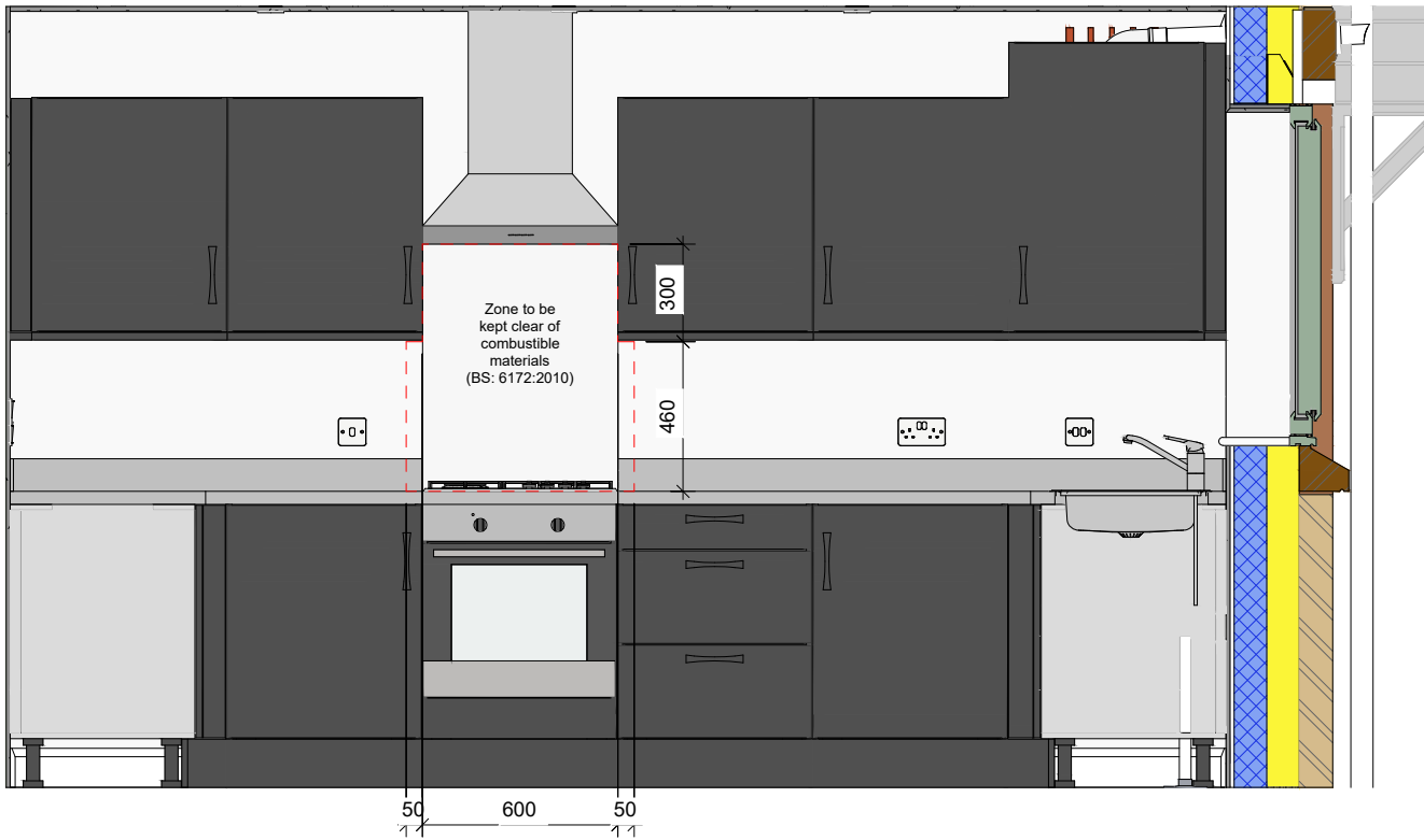
3 Kitchen - View C 1 : 25
